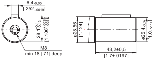
CO - \varnothing 1 " straight, Parallel key \frac{1}{4} "x \frac{1}{4} "x \frac{1}{4} " BS46 Max. Torque 34 daNm [3010 lb-in]
